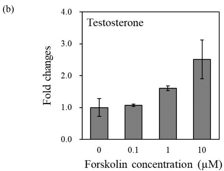
Figure S2. Dose-response curve of forskolin, a positive control. (a) estradiol (E2) content and (b) testosterone content in H295R cell assay.
