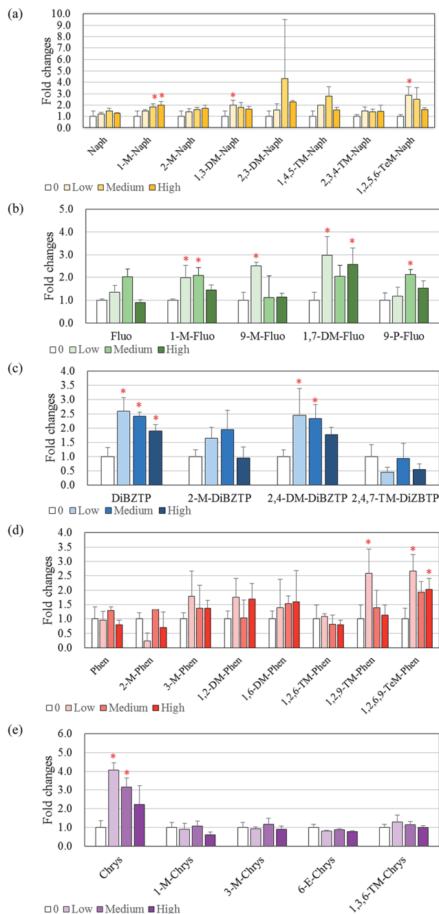
Fig. 3 Effects of unsubstituted and alkylated PAHs on T levels in H295R cells. (a) Naphthalene and alkylated naphthalene, (b) fluorene and alkylated fluorene, (c) dibenzothiophene and alkylated dibenzothiophene, (d) phenanthrene and alkylated phenanthrene, and (e) chrysene and alkylated chrysene. Data are expressed as fold changes compared to appropriate solvent control (means \pm standard deviations ( n = 3 )). Asterisk (*) indicates a significant difference from the solvent control ( p < 0.05 ).
