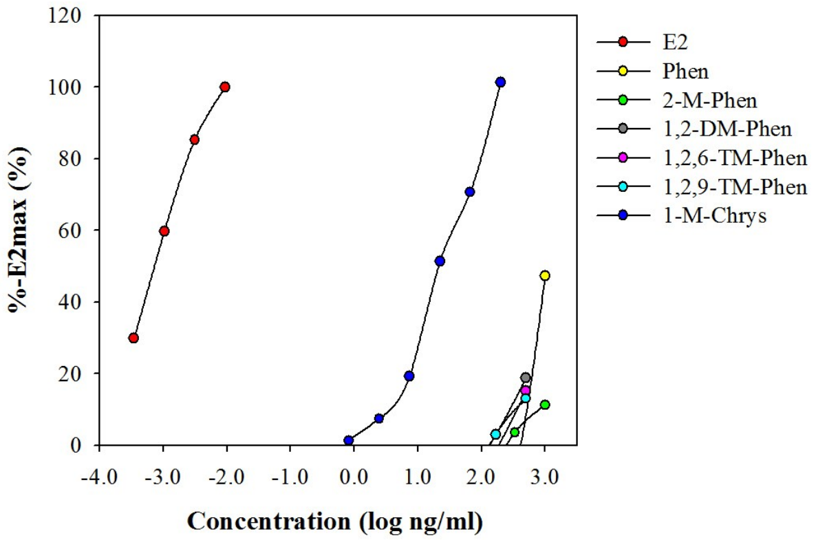
Figure S3. Dose dependent ER-mediated potencies observed from several PAHs with >10% ER-mediated potency.
