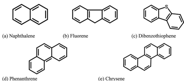
Fig. 1 Chemical structures of tested unsubstituted PAHs.
