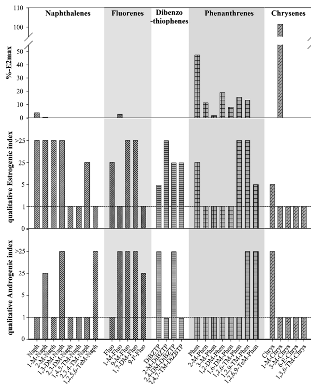
Fig. 4 %E2-max, qEI (qEI = NOEC of cell survival/NOEC of changes in E2 concentration), and qAI (qAI = NOEC of cell survival/NOEC of changes in T concentration) of tested PAHs. qEIs or qAIs are used to compare relative estrogenic or androgenic potential among PAHs.
