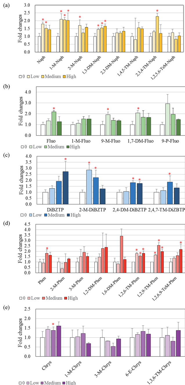
Fig. 2 Effects of unsubstituted and alkylated PAHs on production of E2 by H295R cells. (a) Naphthalene and alkylated naphthalene, (b) fluorene and alkylated fluorene, (c) dibenzothiophene and alkylated dibenzothiophene, (d) phenanthrene and alkylated phenanthrene, and (e) chrysene and alkylated chrysene. Data are expressed as fold changes compared to appropriate solvent control (means \pm standard deviations ( n = 3 )). Asterisk (*) indicates a significant difference from the solvent control ( p < 0.05 ).
