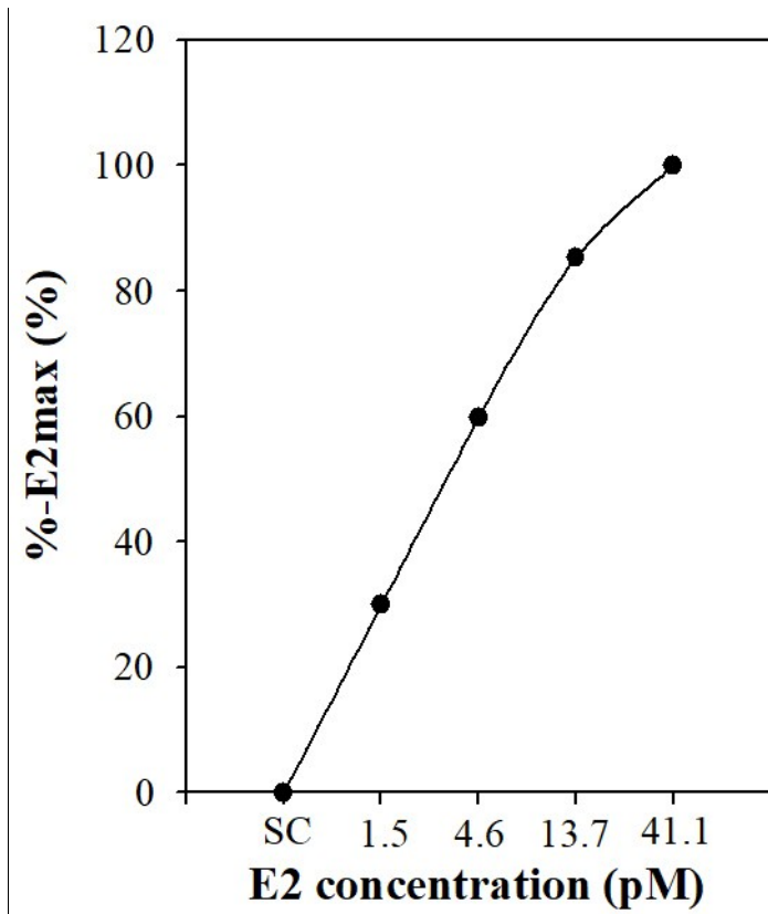
Figure S1. Dose-response curve of estradiol (E2), a positive control used for MVLN- luc assay.
