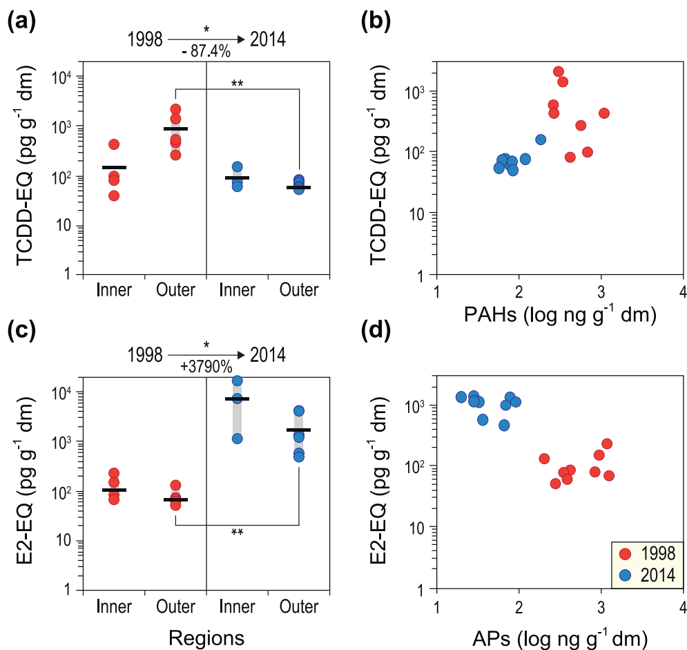
Fig. 3. Spatiotemporal distributions of (a) TCDD-EQ and (c) E2-EQ biological responses in inner- and outer-region Masan Bay sediment samples for 1998 and 2014. (b and d) Scatter plots showing dose-response relationships between chemical contaminant levels and biological responses in sediment samples collected from Masan Bay (* p < 0.05 ).
