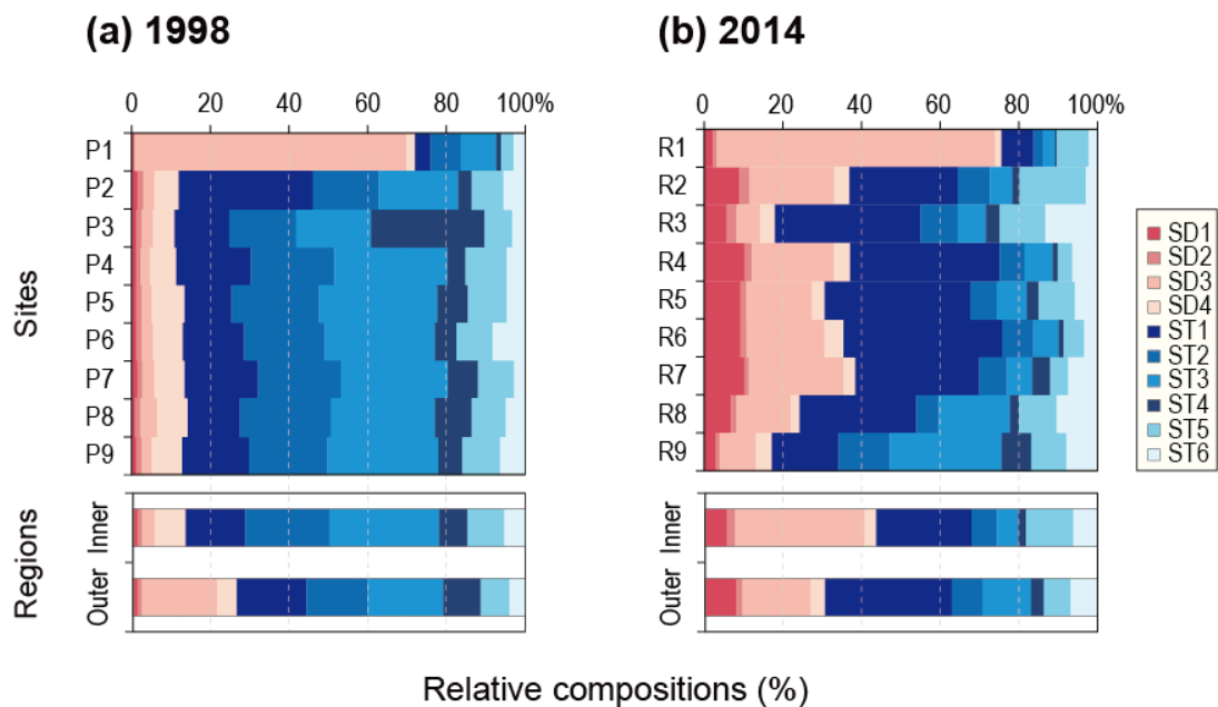
Fig. S2. Comparison of the relative SOs compositions (10 component SOs) at each sampling site and at inner-region versus outer-region sites within Masan Bay.
