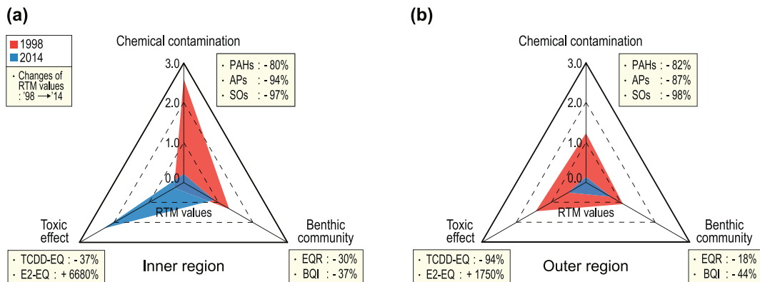
Fig. 5. Sediment quality triads of normalized to RTMVs obtained for chemical contamination, toxic effects, and benthic community quality of sediment samples from (a) inner and (b) outer regions in 1998 and 2014.
