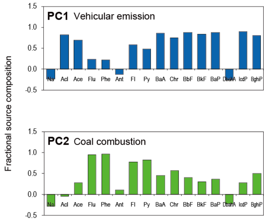
Fig. S1. PCA after Varimax rotation for selected PAHs in Masan Bay sediments.
