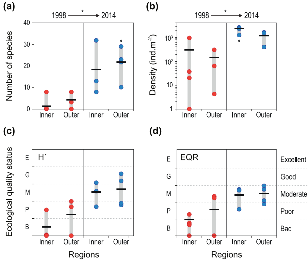
Fig. 4. Recovery of benthic community health in Masan Bay. Comparisons of (a) numbers of taxa (species) and (b) distributions (density, ind. m -2 ) of benthic communities in Masan Bay between 1998 and 2014. Comparisons of EcoQ status as represented by (c) the Shannon-Wiener (H') index and (d) the EQR in Masan Bay between 1998 and 2014 (* p < 0.05).
