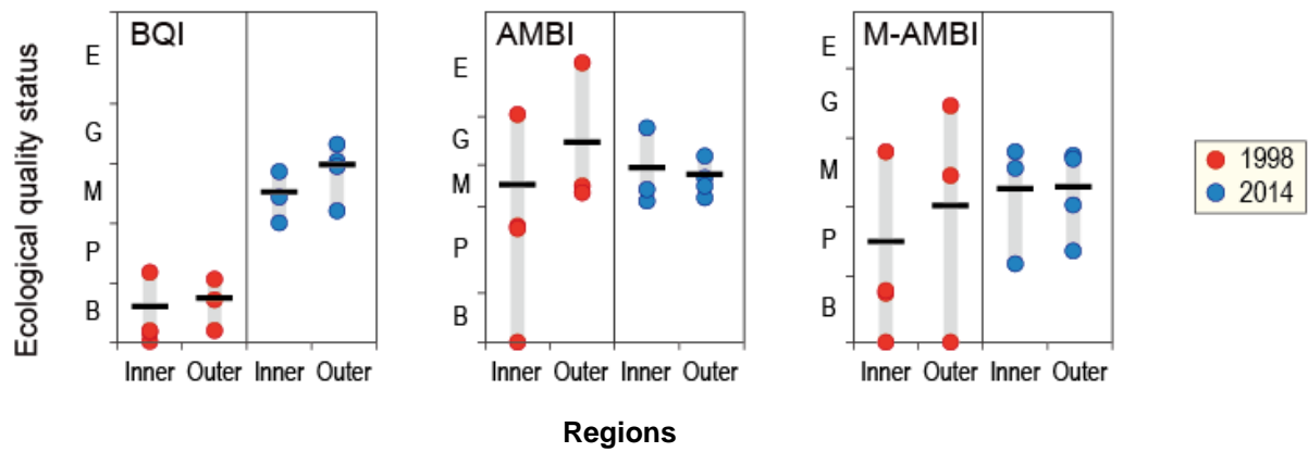
Fig. S3. Ecological quality (EcoQ) status as indicated by Benthic Quality Index (BQI), Azti Marine Biotic Index (AMBI), and Multivariate-AMBI (M-AMBI) indices.
