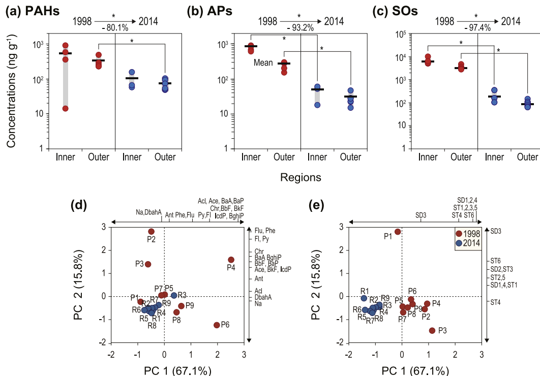
Fig. 2. Concentrations of (a) PAHs, (b) APs, and (c) SOs in sediment from Masan Bay in 1998 and 2014. Cluster results from PCA of (d) PAH and (e) SO concentrations in sediments collected from 18 locations in Masan Bay. Percentages of variability in each data accounted for by PC 1 and PC 2 are shown in the graph (* p < 0.05 ).
