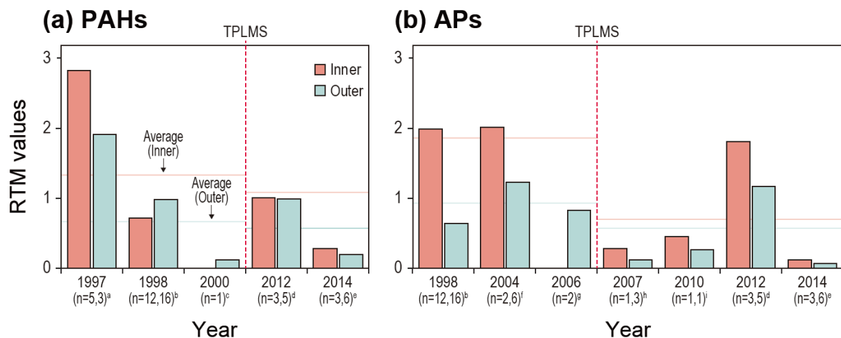
Fig. S4. Comparisons of normalized RTMVs for (a) PAHs and (b) APs in sediments of inner and outer regions of Masan Bay obtained from this study and previous studies (Data from a Yim et al., 2005; b Khim et al., 1999a; c Moon et al., 2001; d Jung et al., 2012; e This study; f Li et al., 2008; g Hong et al., 2009; h Choi et al., 2009; and i Al-Odaini et al., 2005).
